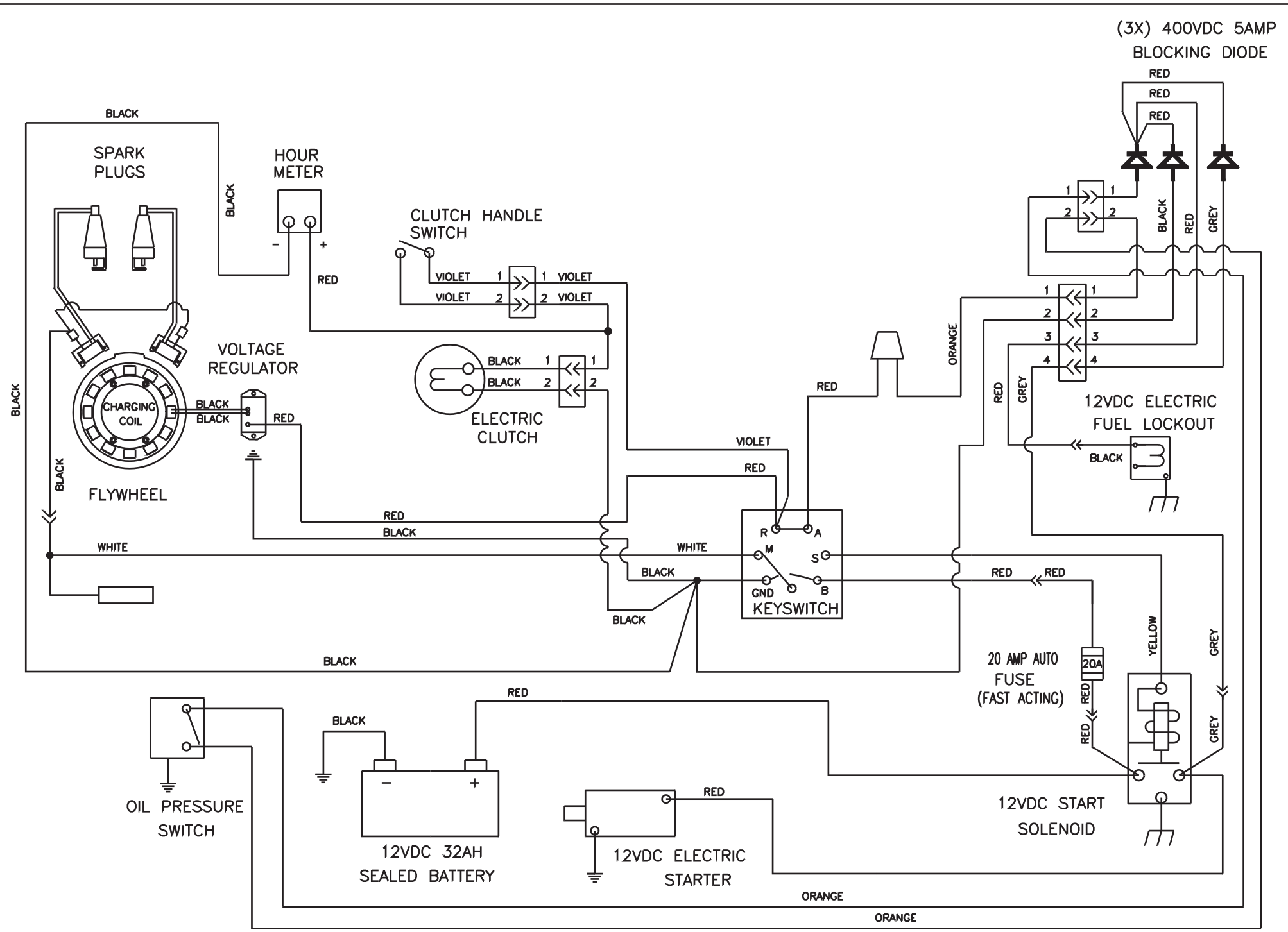
ELECTRICAL SCHEMATIC
